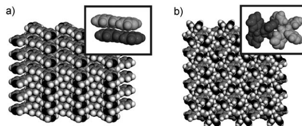
Figure 6. Accessibility of N atoms (black): a) olefin 4,4'-bpe and b) photoproduct 4,4'-tpcb along (-101) and (001) planes, respectively. Insets show localized packings.
